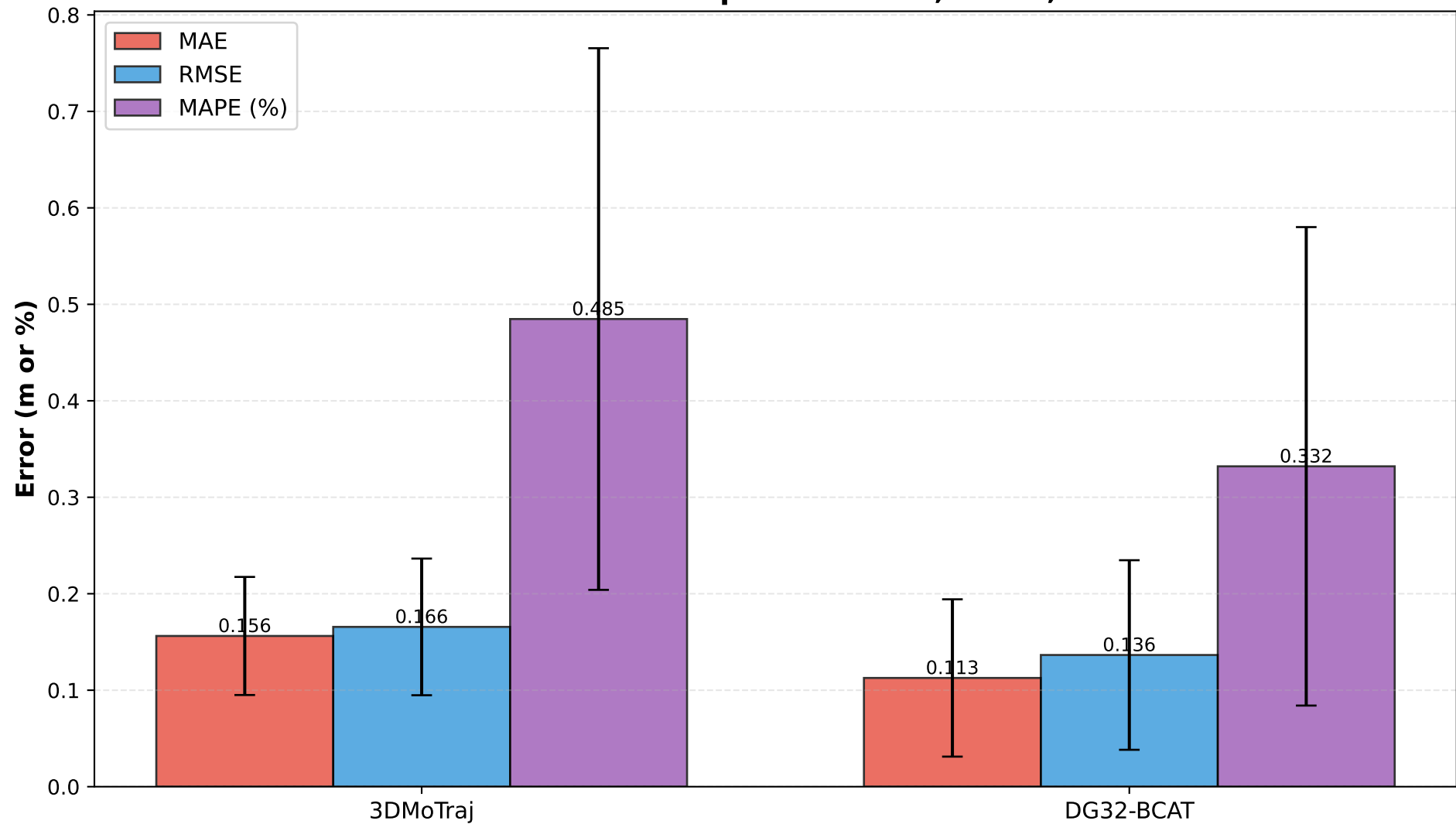
Overall Metrics Comparison: MAE, RMSE, MAPE
